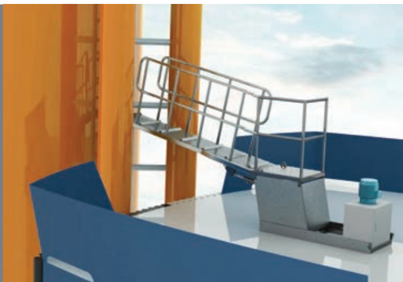
DYNAMIC OFFSHORE GANGWAY FOR ACCESS TO WIND TURBINES
